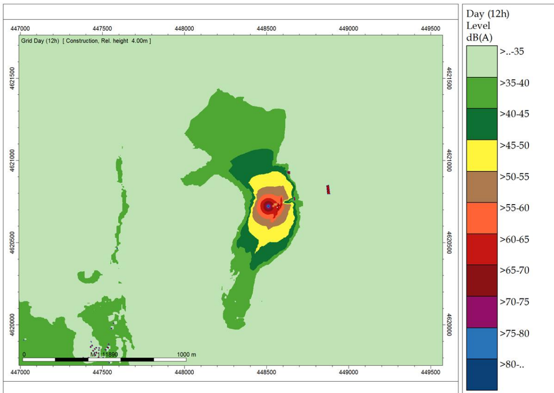
Figure J-3: Noise Propagation Model for Construction Phase (Shaft 3)
