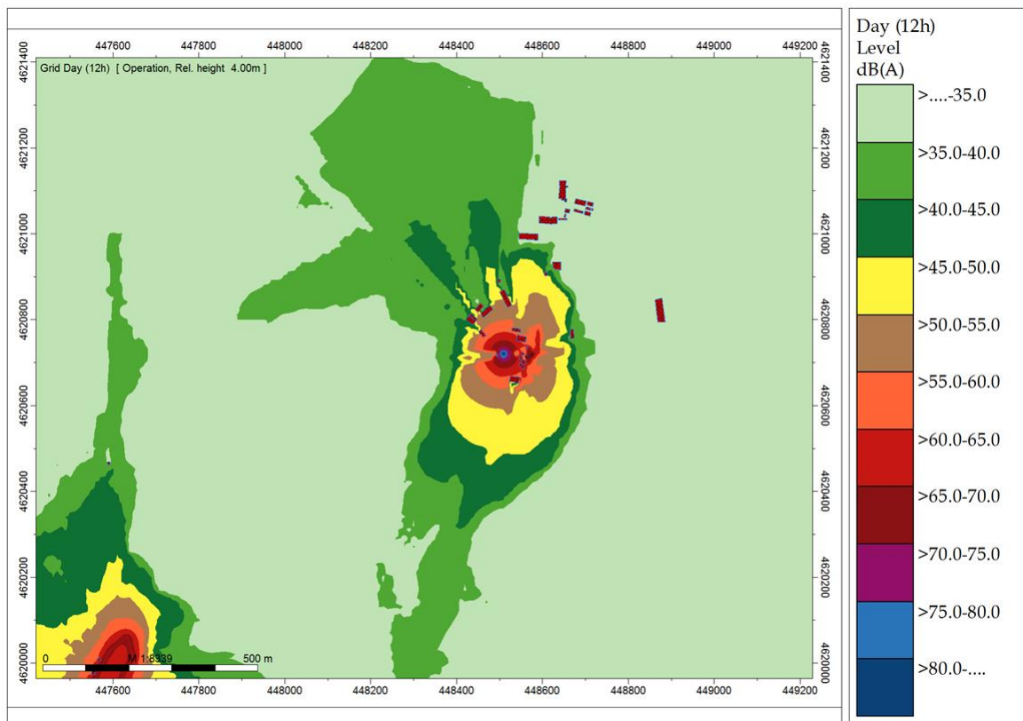
Figure J-6: Noise Propagation Model for Operation Phase (Shaft 3)
