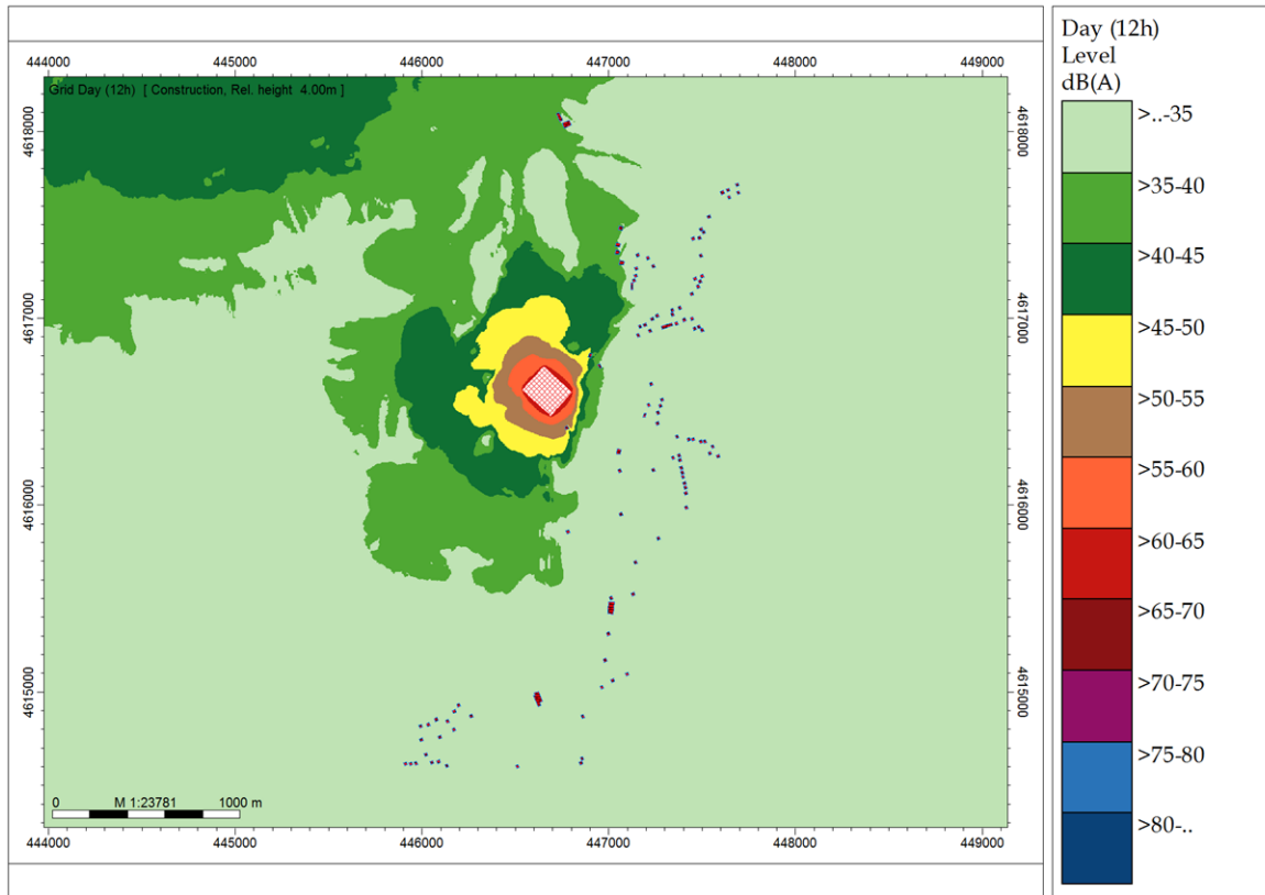
Figure J-2: Noise Propagation Model for Construction Phase (Shaft-2)
