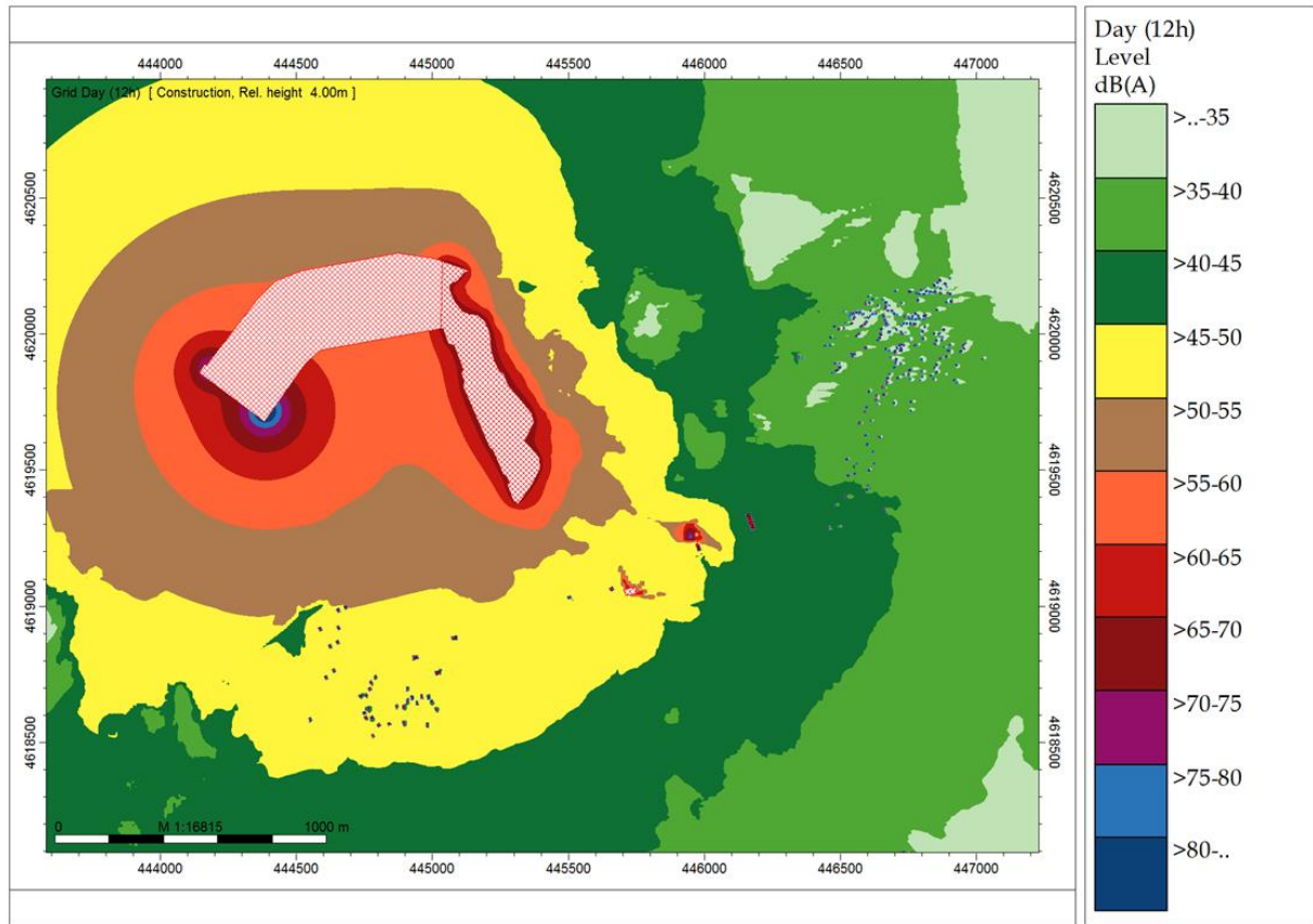
Figure J-1: Noise Propagation Model for Construction Phase (Shaft-1)
