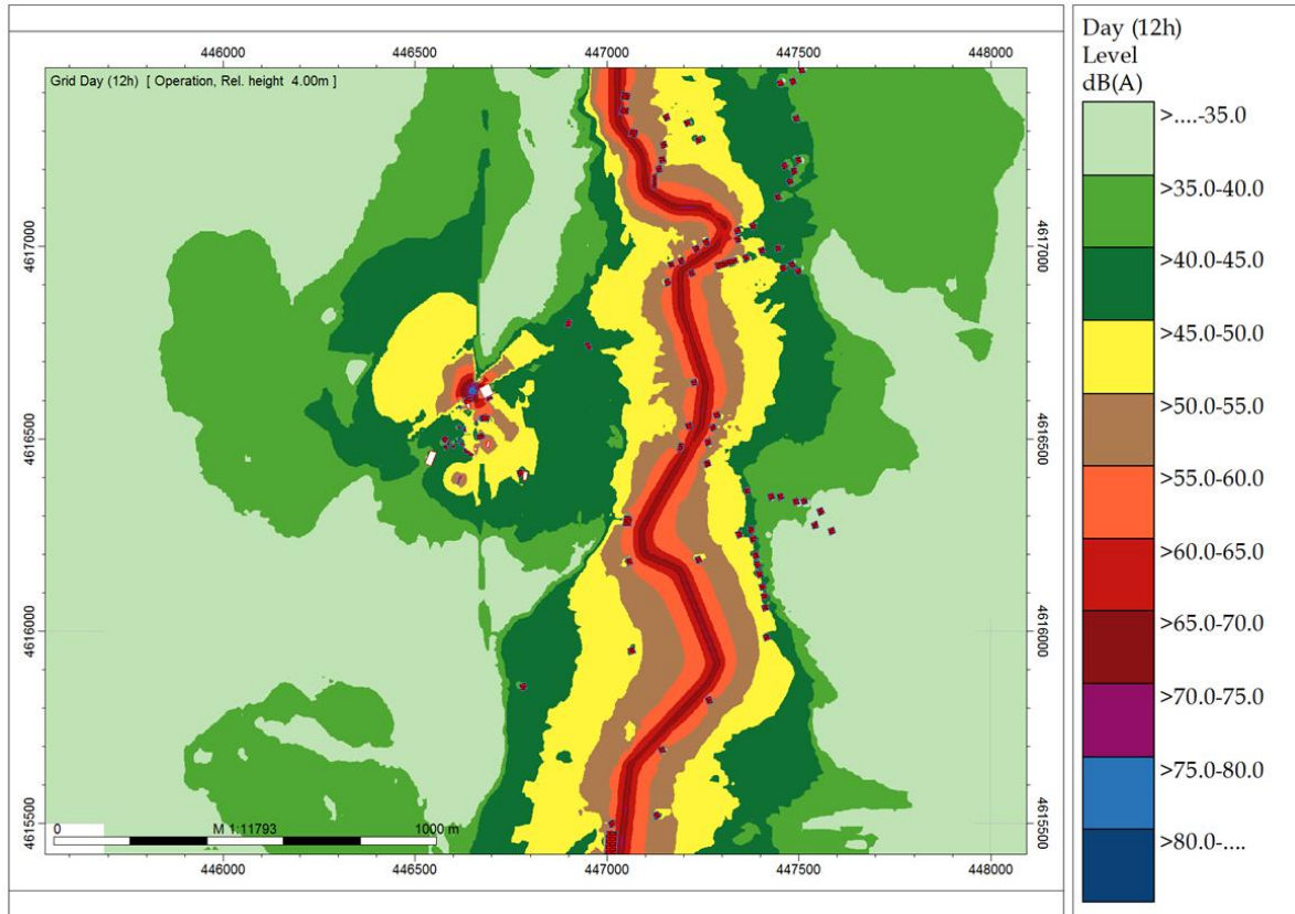
Figure J-5: Noise Propagation Model for Operation Phase (Shaft 2)
