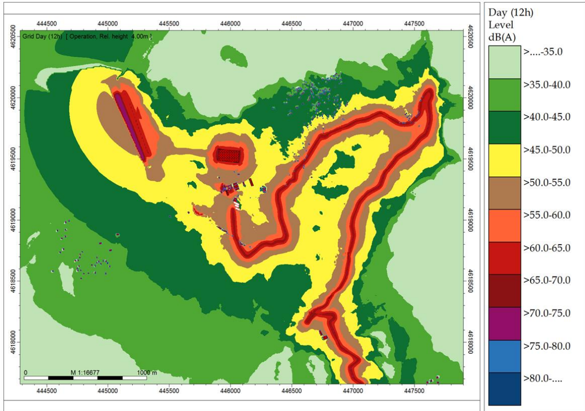
Figure J-4: Noise Propagation Model for Operation Phase (Shaft 1)
